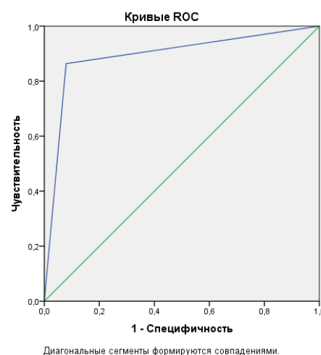
Fig.2.-ROC curve characterizing the sensitivity and specificity of the method for assessing the likelihood of developing postoperative arrhythmias by the concentration of free hemoglobin in blood plasma.
